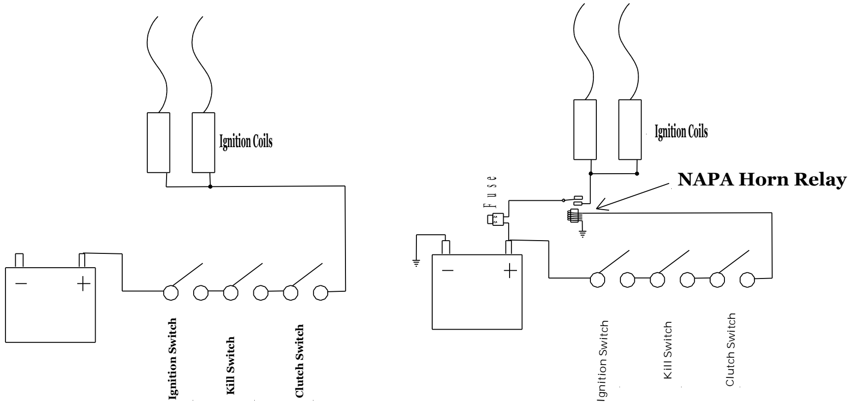
Stock Wiring with Relay
